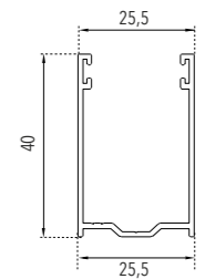
ART. GU40 Guida in alluminio A40 25,5X40 mm
